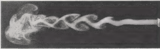
▲ In the open sea mighty vortices can arise in which the whole dynamic force of the suction centre becomes visible.
